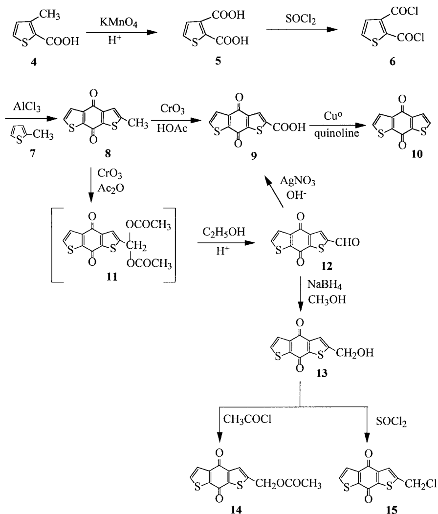
Scheme 1. Synthesis of 2-methyl-4,8-dihydrobenzo[1,2- b :5,4- b' ]dithiophene-4,8-dione ( 8 ) and its derivatives.
