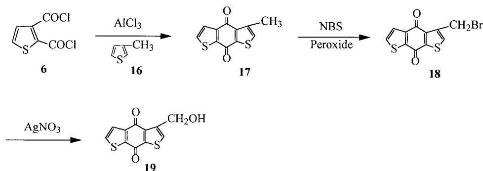
Scheme 2. Synthesis of 3-methyl-4,8-dihydrobenzo[1,2- b :5,4- b' ]dithiophene-4,8-dione (17) and its derivatives.
